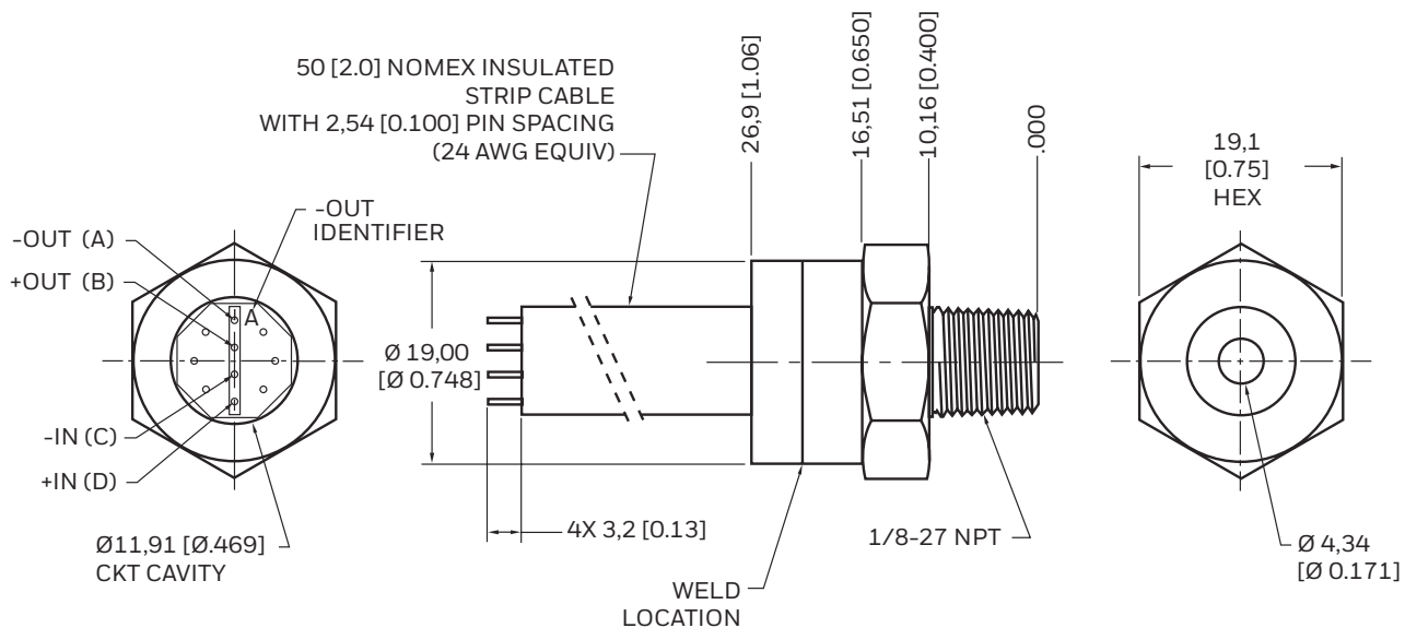
Figure 3. Package 4: 1/8-27 NPT
