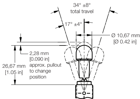
Locking lever dimensions for four-pole TL toggles
