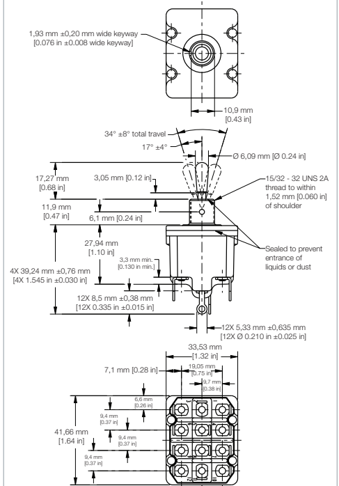
14NT1: Four-pole, standard lever, solder terminals
