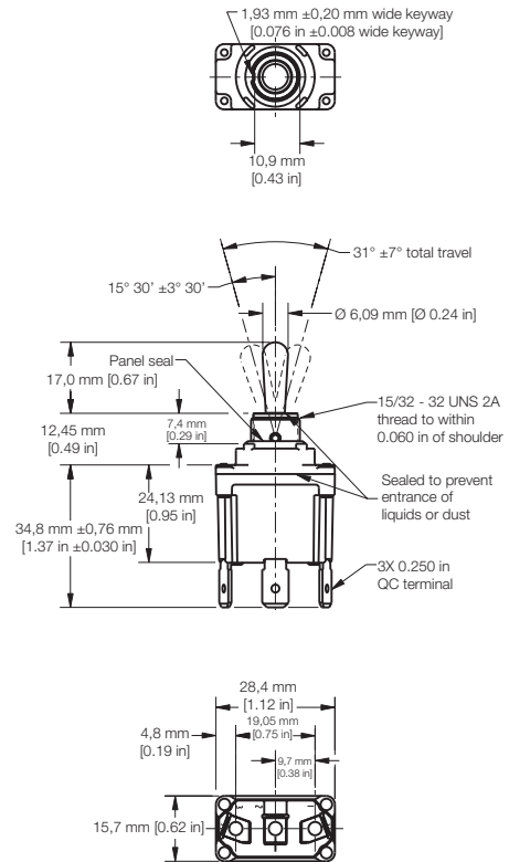
632NT91: standard lever, panel standoff, quick-connect terminals
