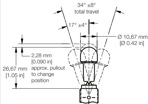
Locking lever dimensions for four-pole NT toggles
