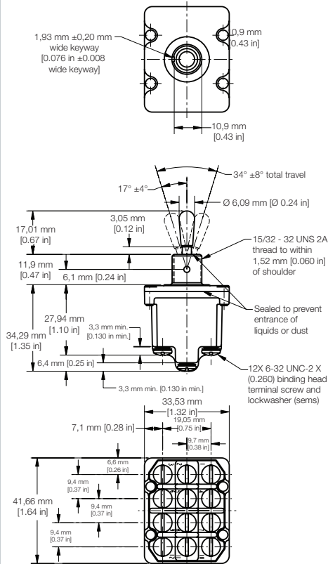
Locking lever dimensions for four-pole NT toggles
