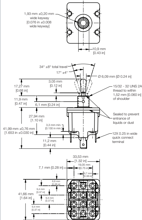
4NT91: Four-pole, standard lever, quick-connect terminals
