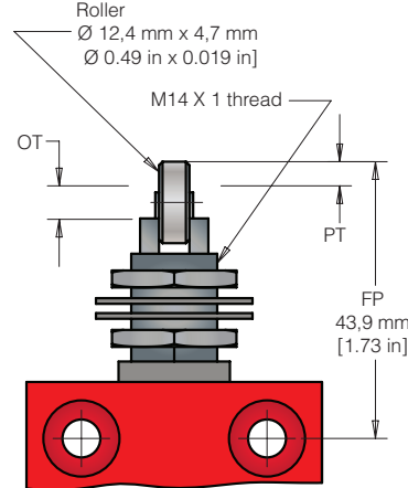
Figure 10. 924CE29 Dimensions
